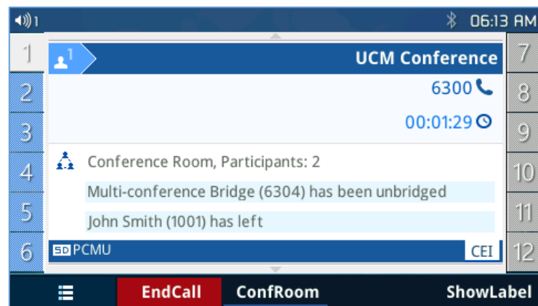
Figure 62: Conference Unbridge
