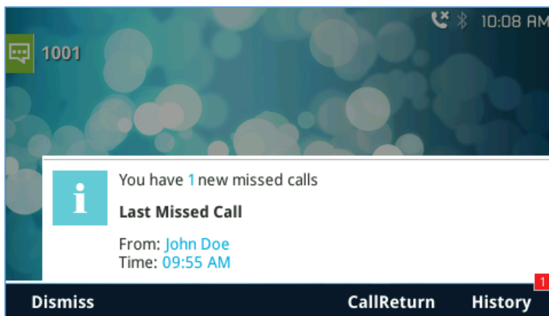
Figure 66: Missed Calls
