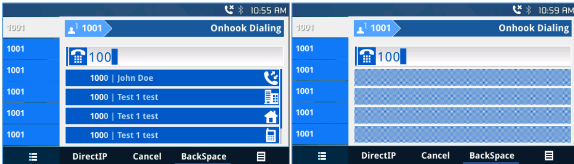
Figure 35: Predictive Dialing
