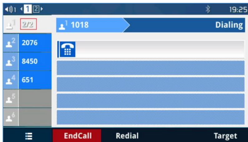
Figure 53: Account Mode
