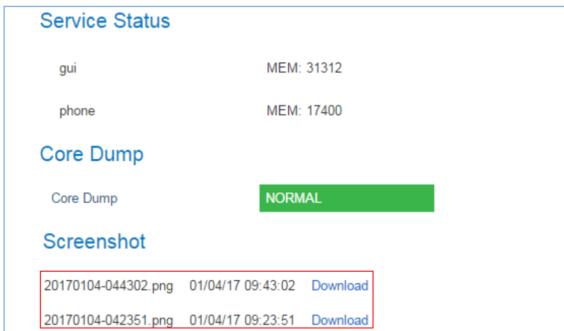
Figure 67: Screenshots
