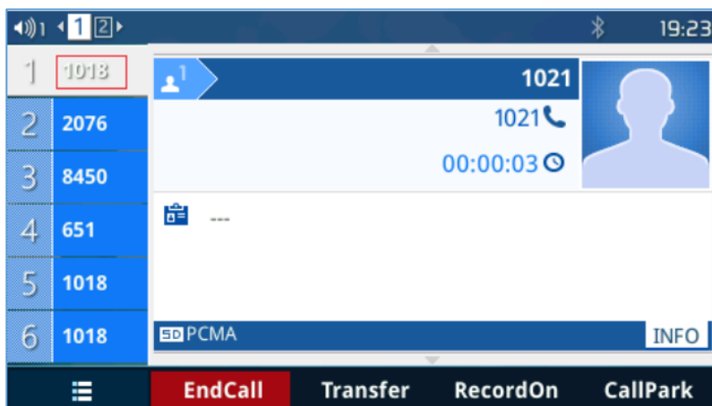
Figure 52: Line Mode
