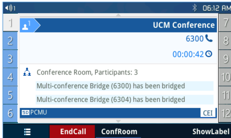
Figure 61: Conference Bridge
