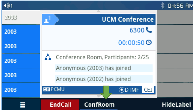
Figure 57: ConfRoom Softkey
