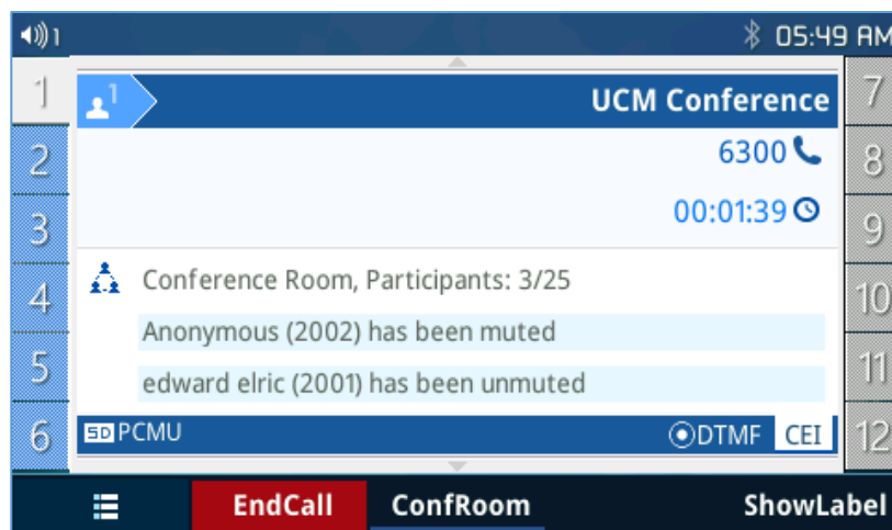
Figure 60: Mute/Unmute Conference
