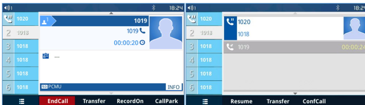
Figure 51: Line Switching
