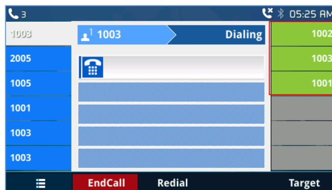
Figure 49: VPK Paging
