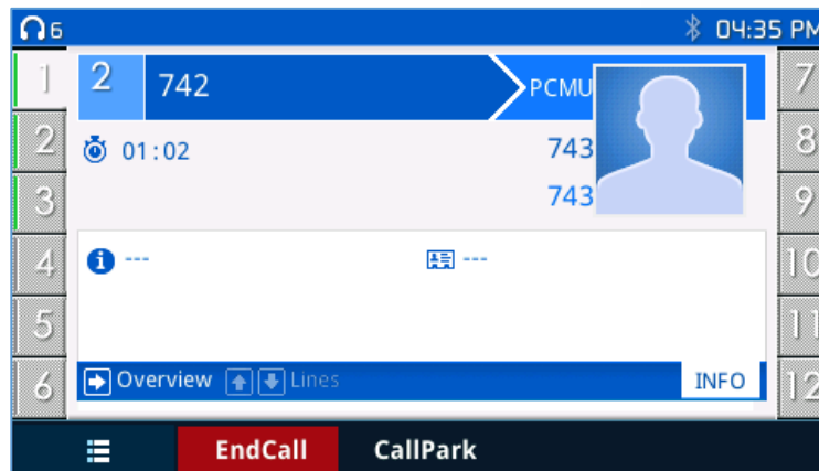
Figure 20: Making Call
